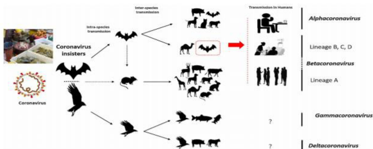
Fig. 2. The key reservoirs and mode of transmission of coronaviruses (suspected reservoirs of SARS-CoV-2 are red encircled); only \alpha and \beta coronaviruses have the ability to infect humans, the consumption of infected animal as a source of food is the major cause of animal to human transmission of the virus and due to close contact with an infected person, the virus is further transmitted to healthy persons. Dotted black arrow shows the possibility of viral transfer from bat whereas the solid black arrow represent the confirmed transfer.
