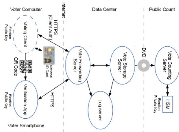
Figure. 2: I-voting system overview
